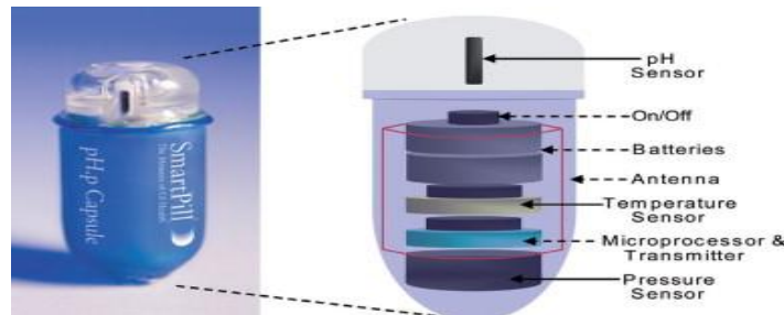
Figure 2: Smartpill components
